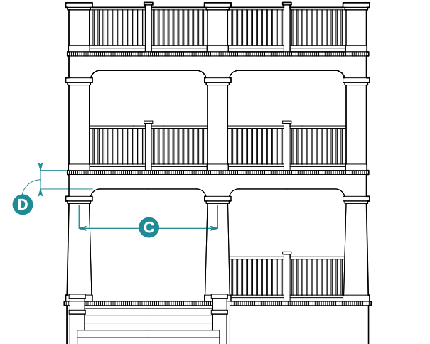
Two-Story Porch with Deck Above
