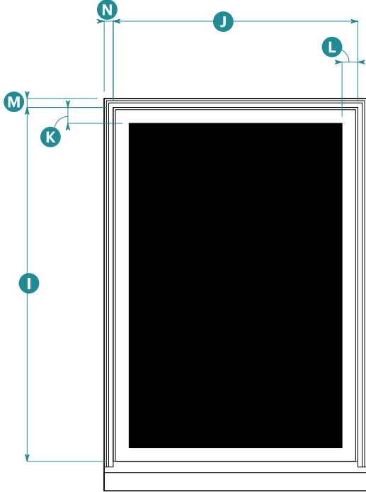
Ground Floor Picture Window Elevation
